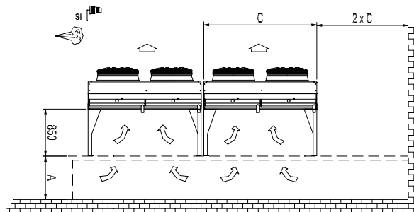
HORIZONTAL INSTALLATION
