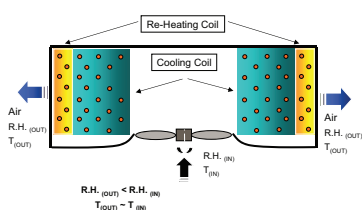
Re heating coil for Dual Discharge
