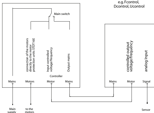
Current distribution with main switch and manual bypass
