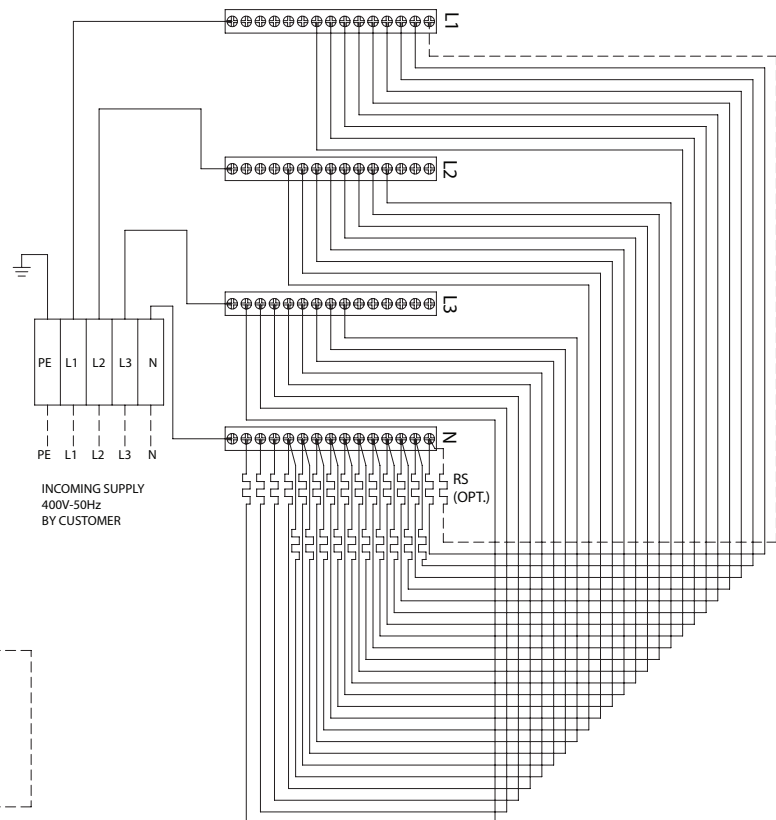
CONNECTION DIAGRAM
