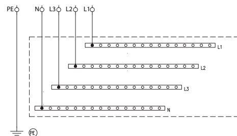
WIRING DIAGRAM
