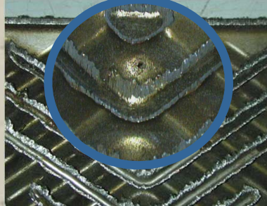
316 corrosion
