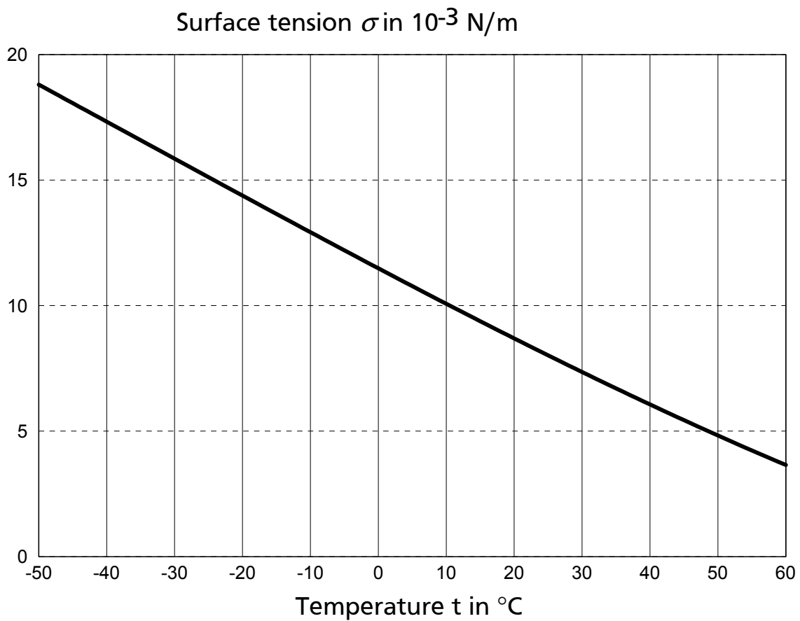
Figure 5: Surface tension
