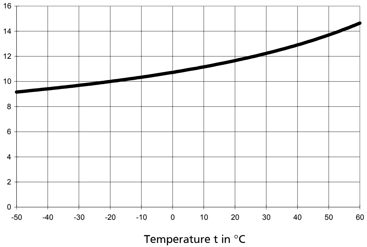
Figure 2: Dynamic viscosity of saturated vapour
