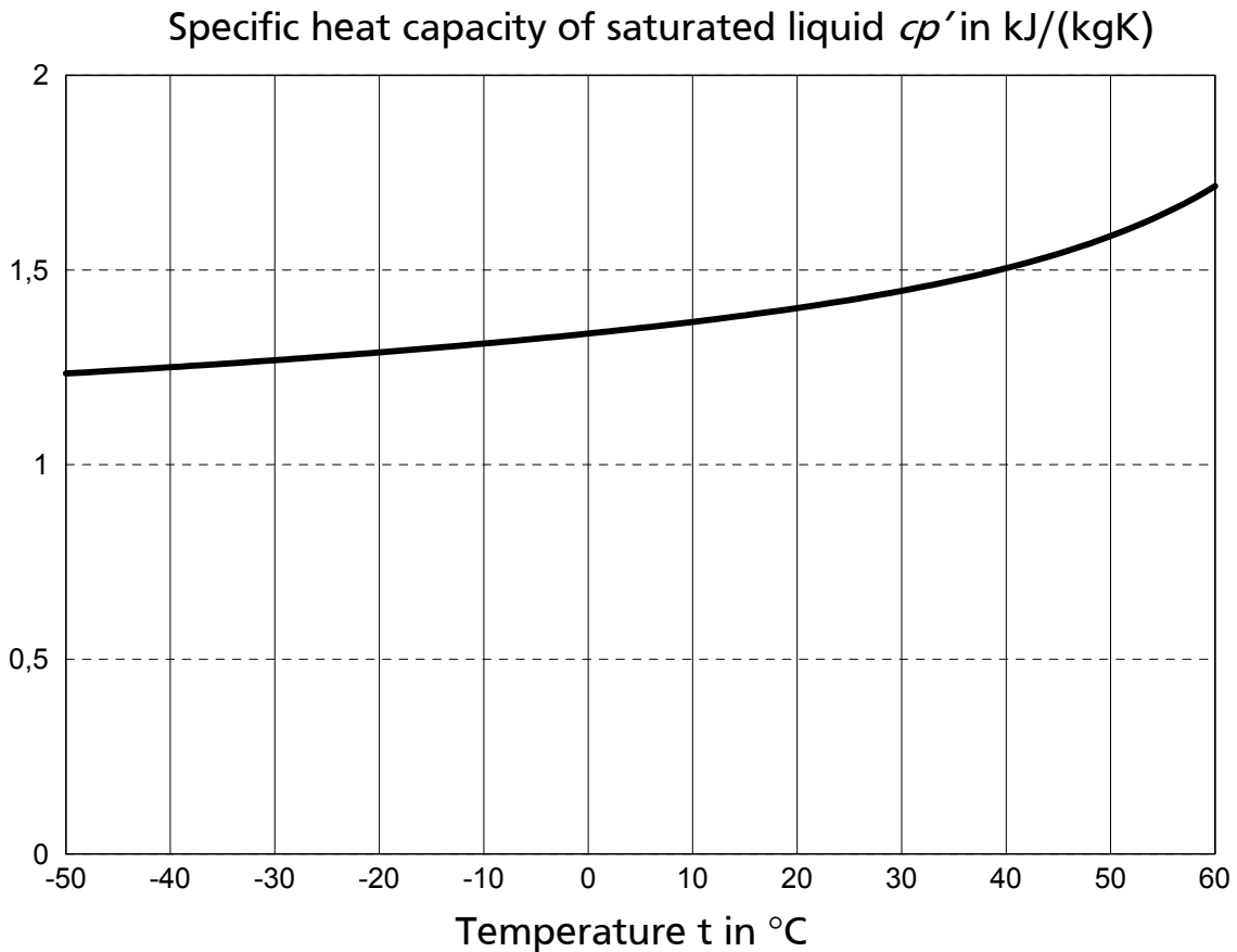
Figure 6: Specific heat capacity of saturated liquid
