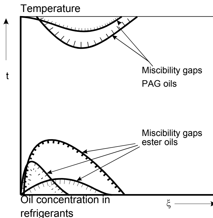
Figure 7: An example of a depiction of miscibility gaps from different types of synthetic lubricants.
